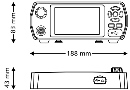
4050 D remote control head (trunk mount configuration) Weight 0.35 kg
